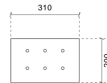
PLAQUE3 (e = 12.0 mm) Échelle 1:10
