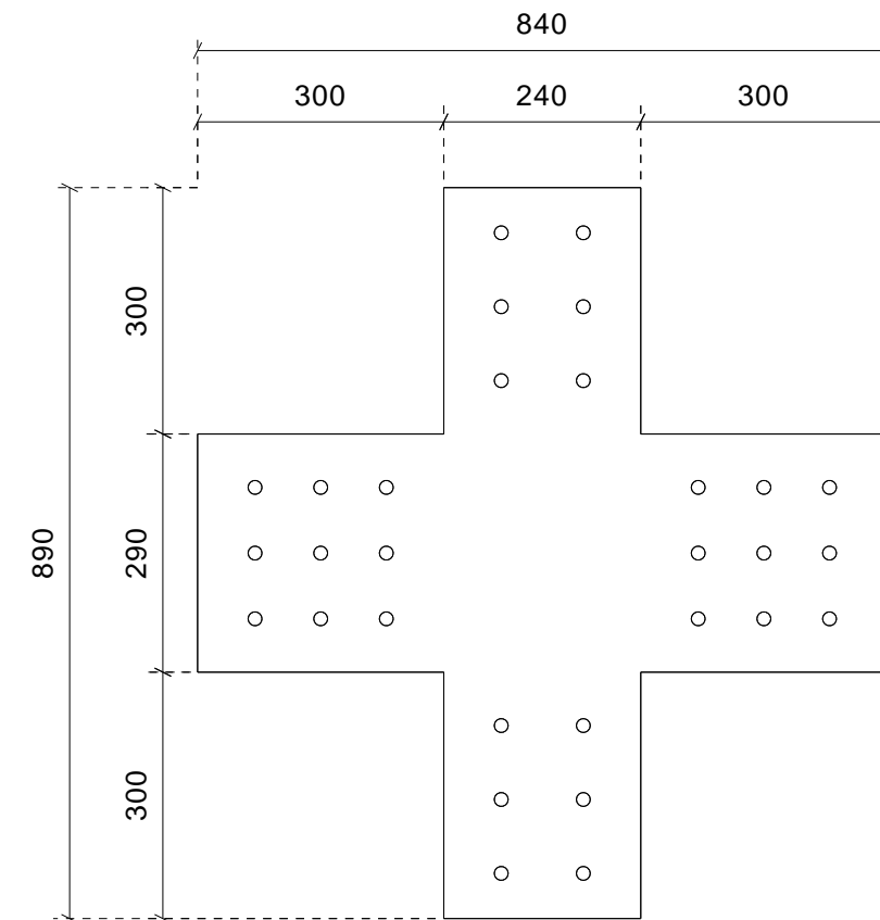
PLAQUE1 (e = 10.0 mm) Échelle 1:10
